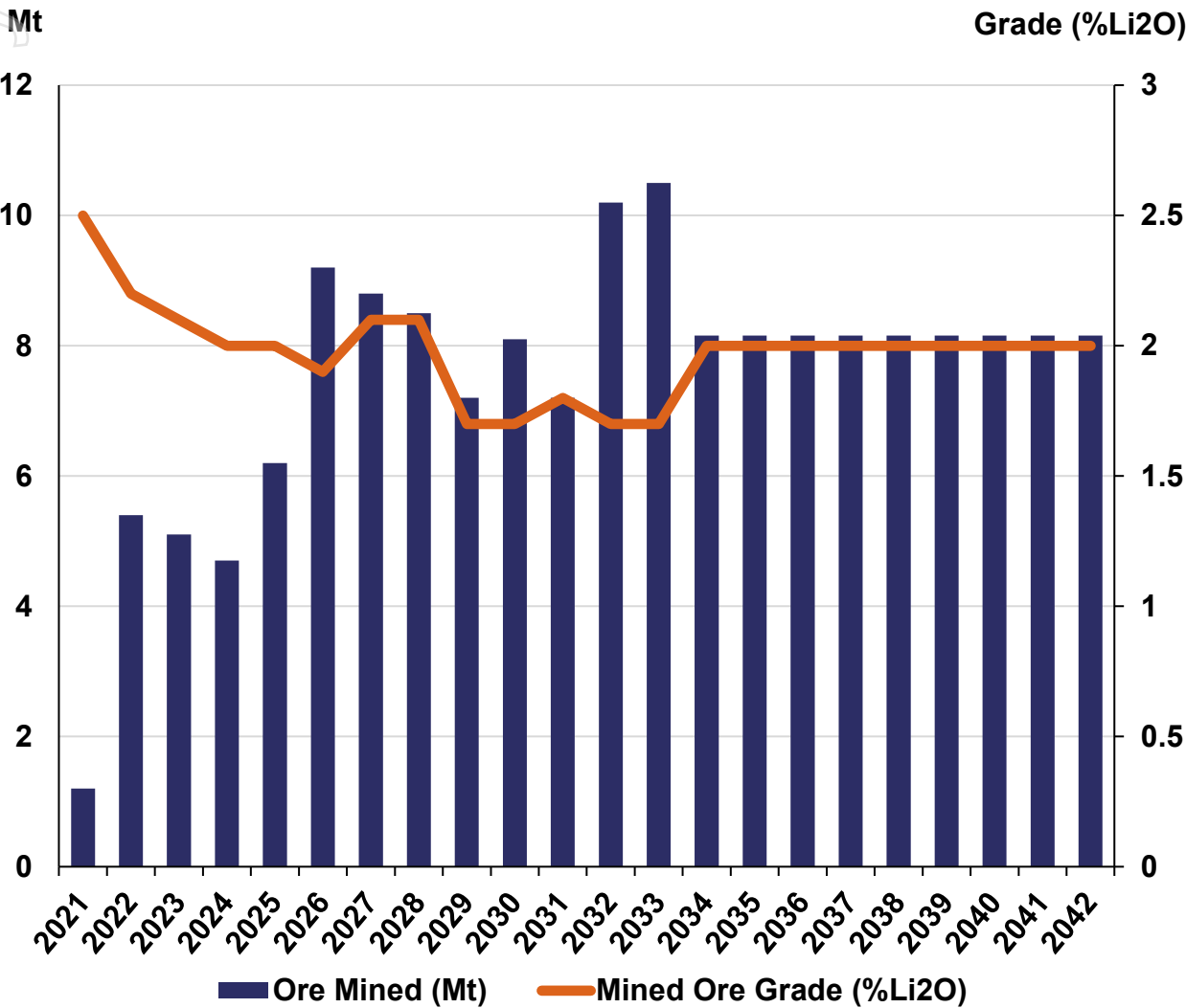
Projected Mined Ore Volume & Grade 1
